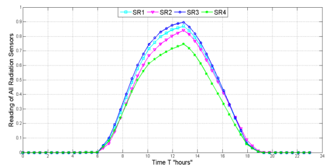
Fig. 16 The measured readings of all radiation sensors S R1 , S R2 , S R3 and S R4
